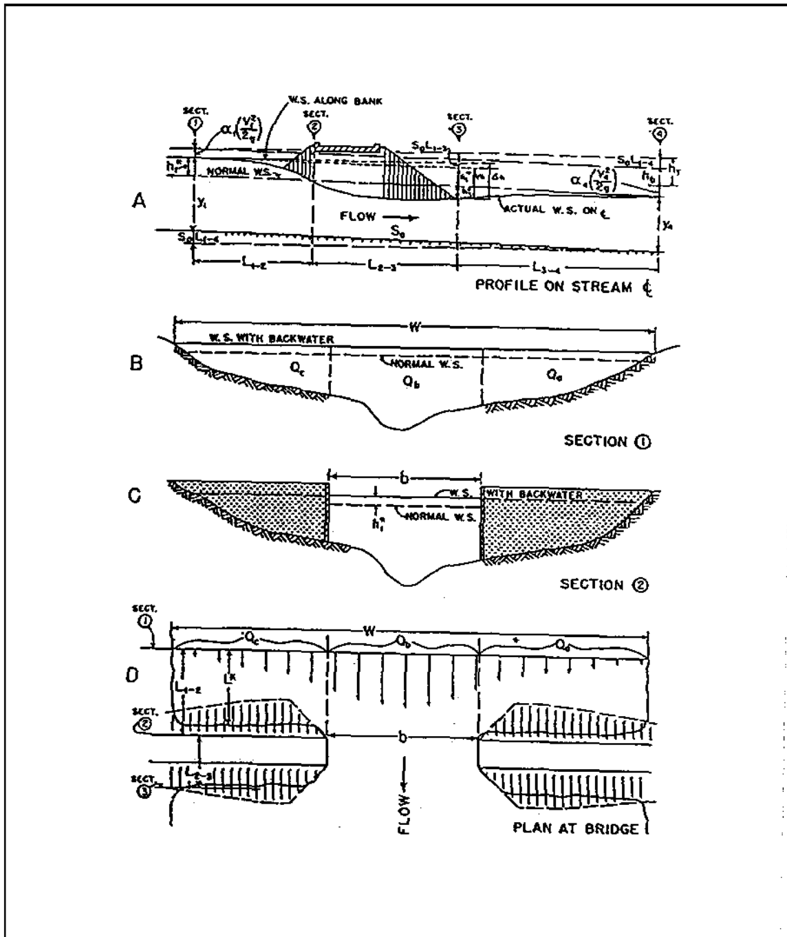
Figure 6-6. Stream profile and cross sections for normal bridge crossing, wingwall abutments
