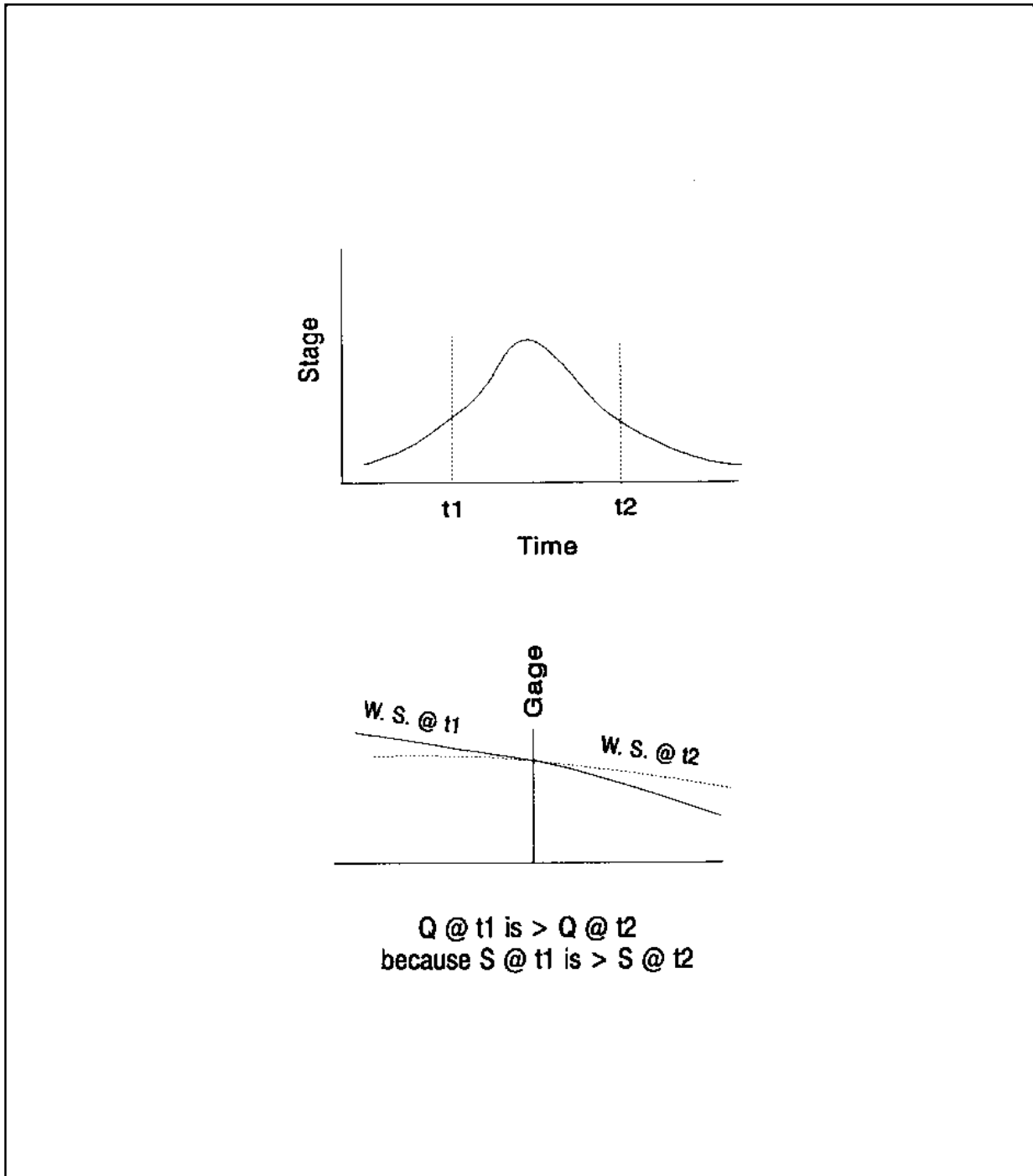
Figure 5-20. Explanation for looped rating curve effect
