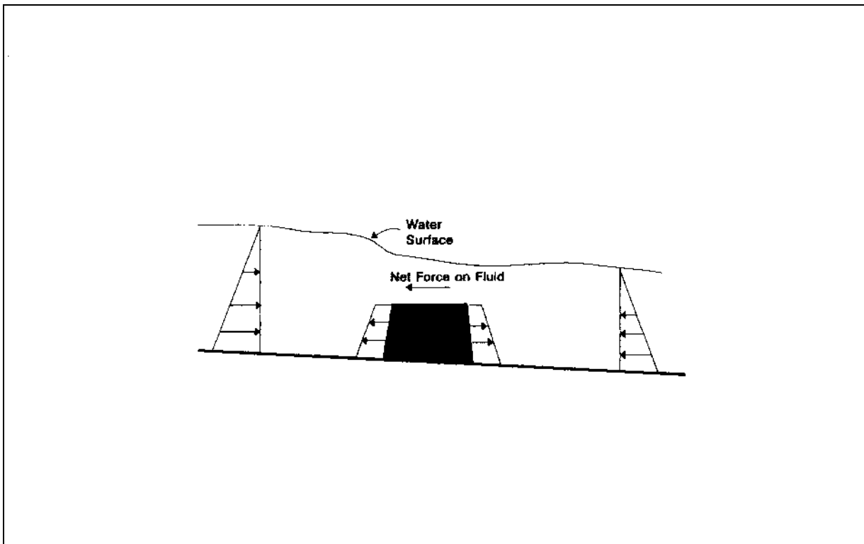
Figure 5-18. Exterior forces acting on a control volume of fluid flowing over a broad crested weir
