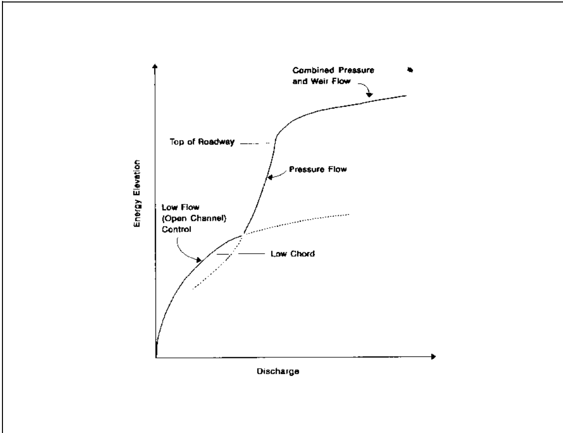
Figure 6-7. Typical discharge rating curve for bridge culvert
