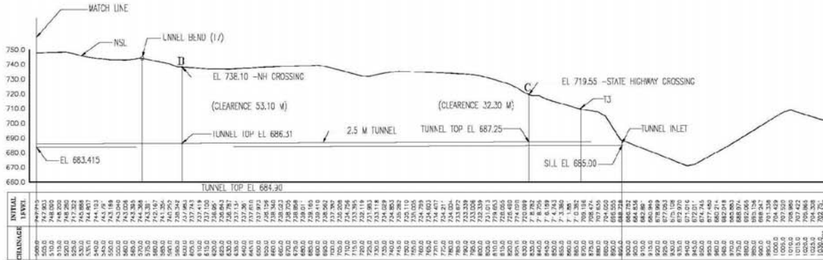
L SECTION OF TUNNEL
