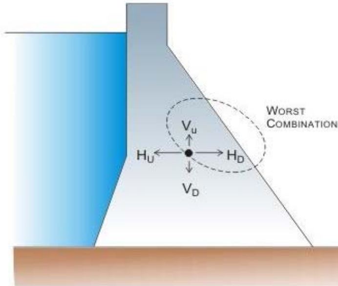
FIGURE 31. Worst combination of earthquake forces under reservoir full condition
