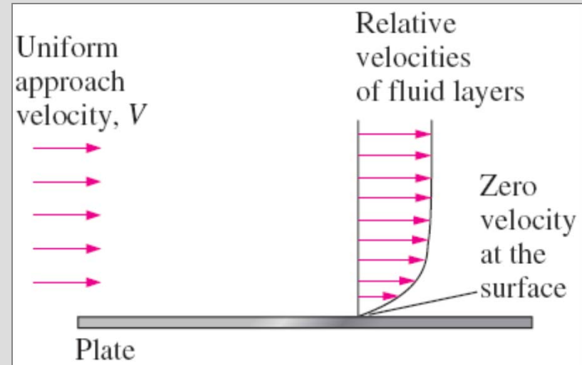
A fluid flowing over a stationary surface comes to a complete stop at the surface because of the no-slip condition.
