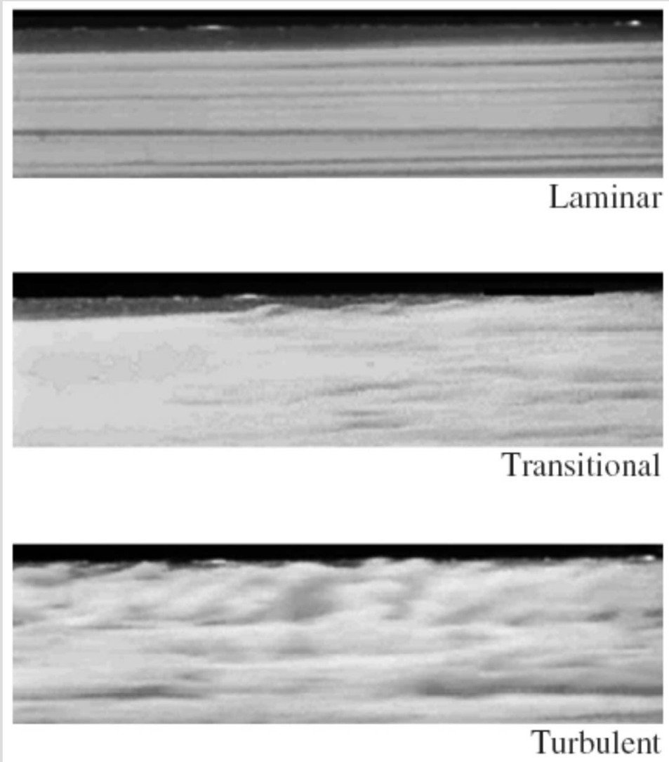
Laminar, transitional, and turbulent flows.
