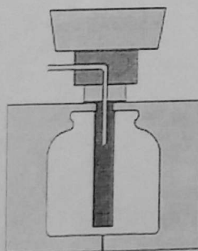
STEP 1 Molten Polymer Material Is Injected Between Two Closed Halves of a Mold
