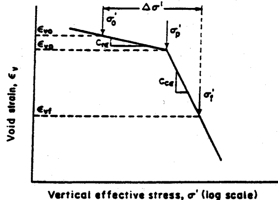
FIGURE 4.4.7.2.3B Typical Consolidation Compression Curve for Overconsolidated Soil-Void Strain Versus Vertical Effective Stress
