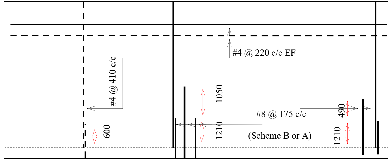
Design of Cantilever Retaining Wall ( This Sketch is not to scale)
